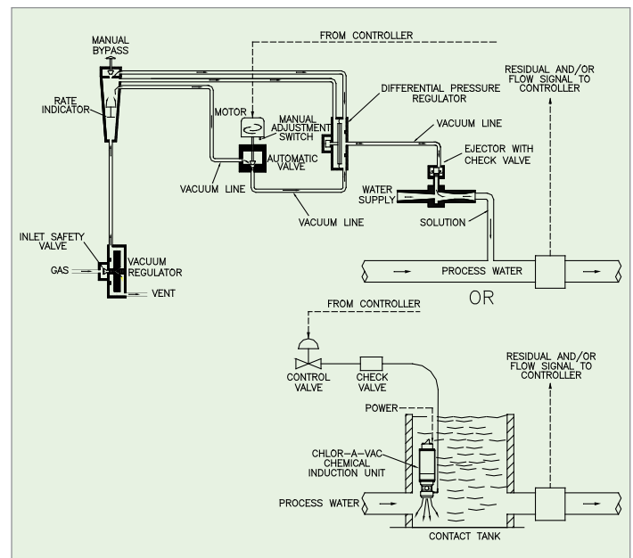
Figure 2 - Model 5240 - Automatic Gas Feed System
