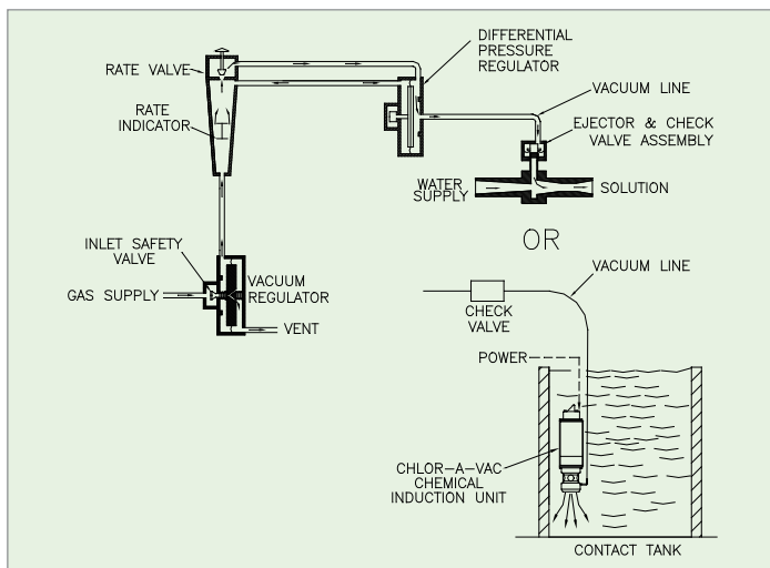
Figure 1 - Model 5210 - Manual Gas Feed System
